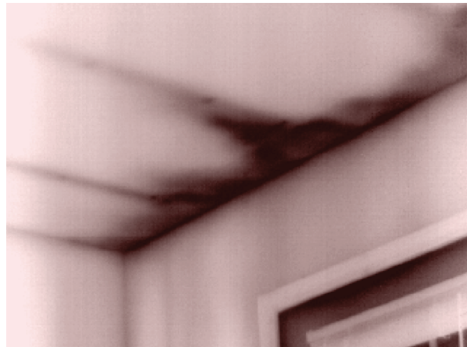
Air wash along the edges of batt insulation produces a unique cold signature on the ceiling of this wood-frame commercial building.
