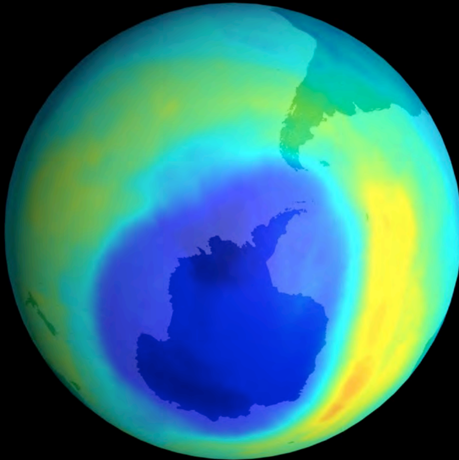
Ozone Hole 1985
